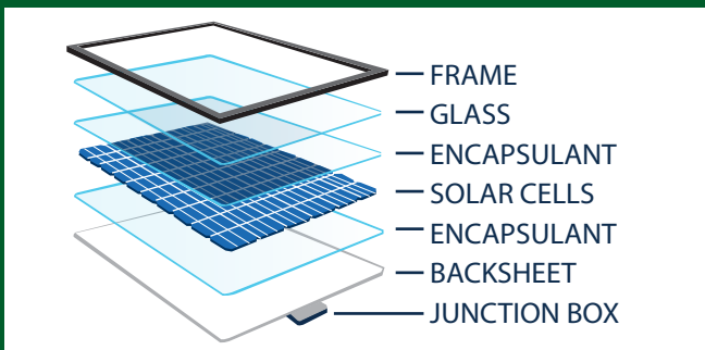
Anatomy of a Solar Panel
